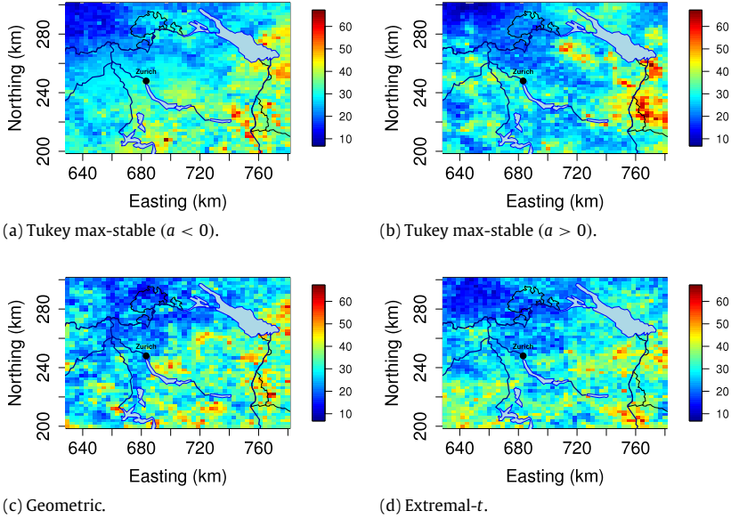
Fig. 4. Realizations of four fitted max-stable processes to the Swiss rainfall data.
