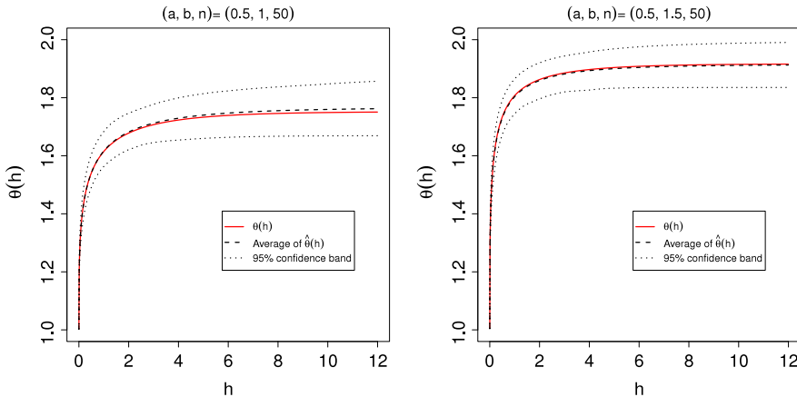
Fig. 2. Estimation accuracy of the extremal coefficient function for the Tukey max-stable process for n = 50 .
