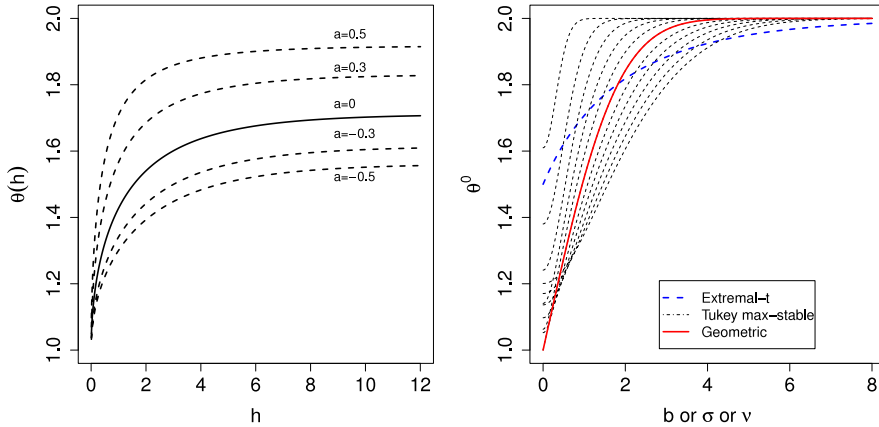
Fig. 1. Bivariate extremal coefficients of various max-stable processes with a Matérn correlation function (12) ( \phi = 3, \nu = 0.5 ). Left: \theta_{TK}(h) for various a 's while fixing b = 1.5 . (Note: a = 0 corresponds to the geometric Gaussian process with \sigma = 1.5 .) Right: \theta_t^0 as a function of v ; \theta_{TK}^0 for 11 values of a equispaced on [-0.9, 0.9] as a function of b ; and \theta_{geo}^0 as a function of \sigma .
