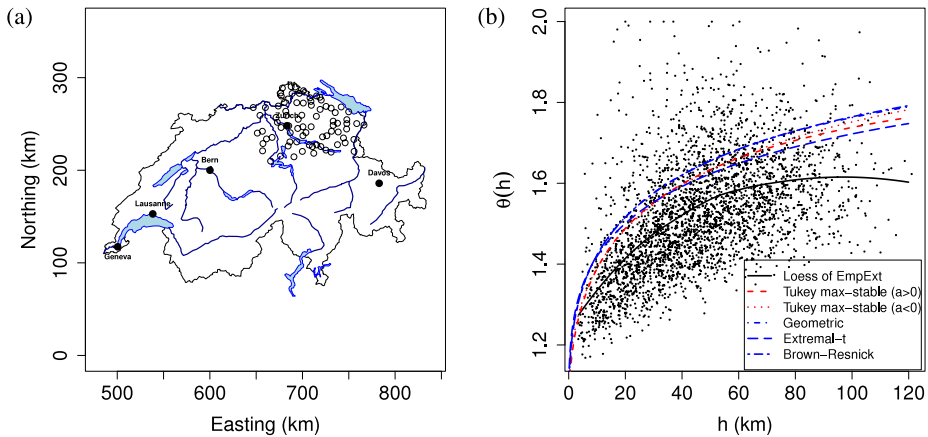
Fig. 3. Swiss rainfall data: (a) Spatial locations of 79 weather stations; (b) Estimated extremal coefficients.
